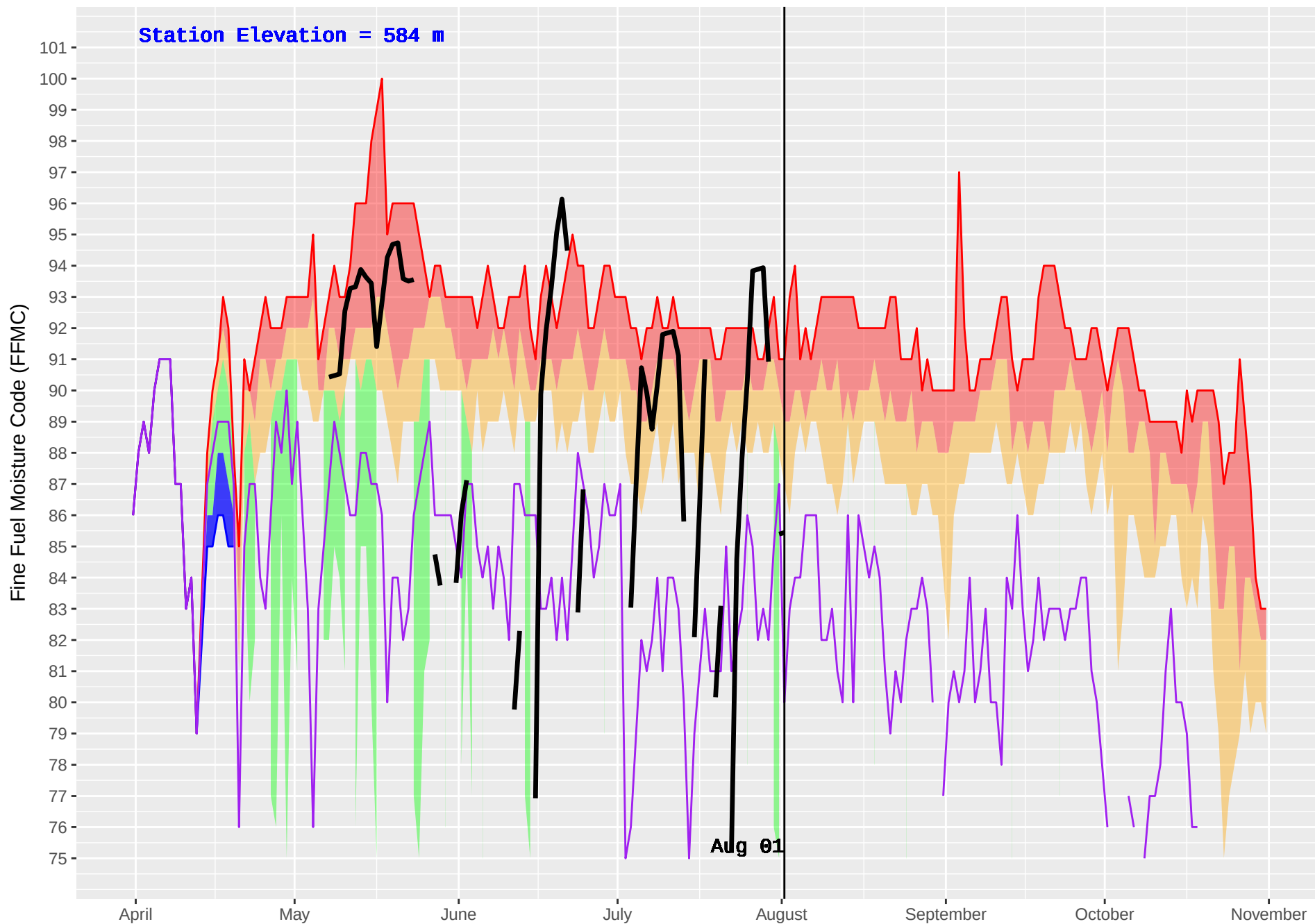
SIERRA (117) : Historical (1981–2016) and Current (2018) Daily Fine Fuel Moisture Code (FFMC)
