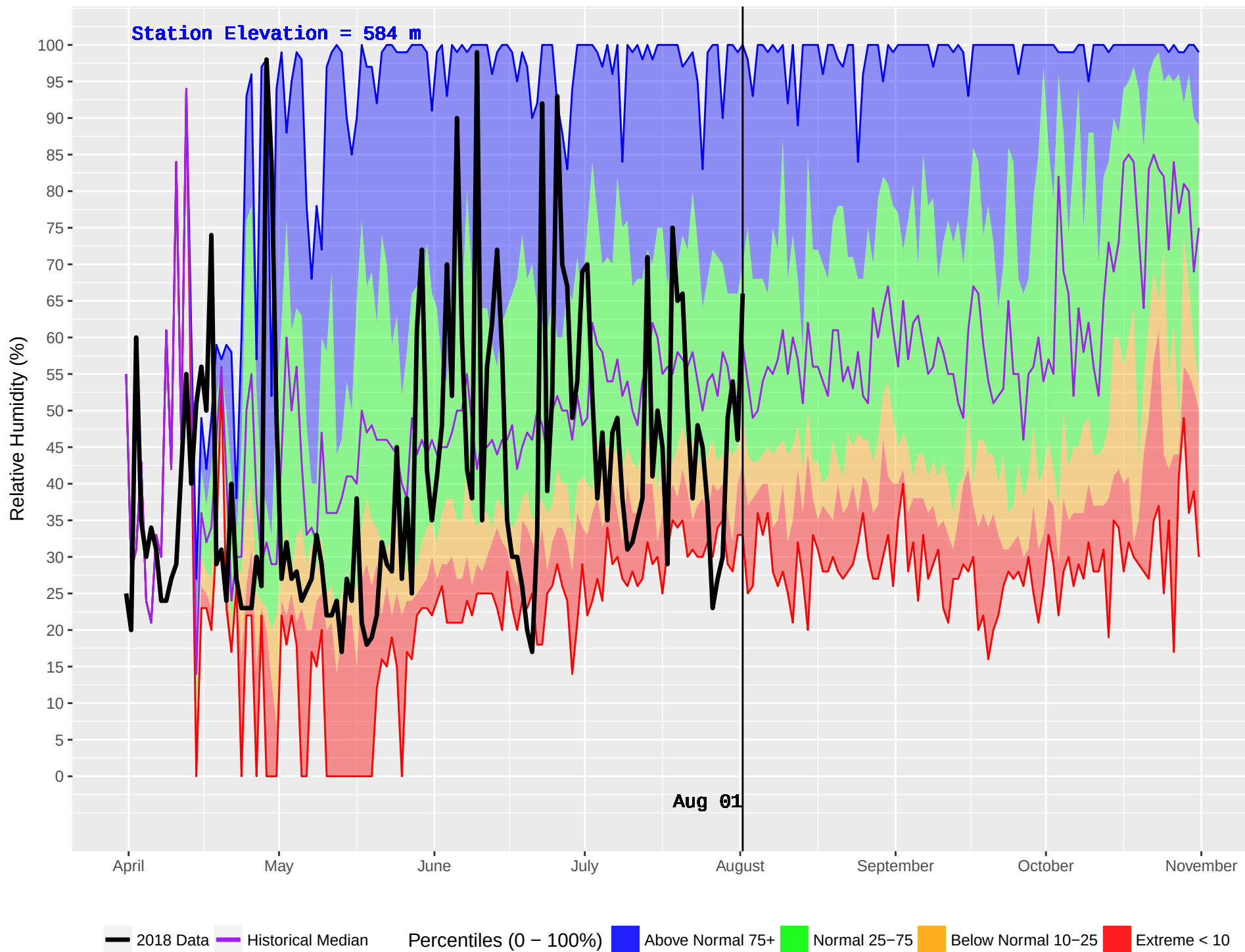
SIERRA (117) : Historical (1981–2016) and Current (2018) Daily Relative Humidity
