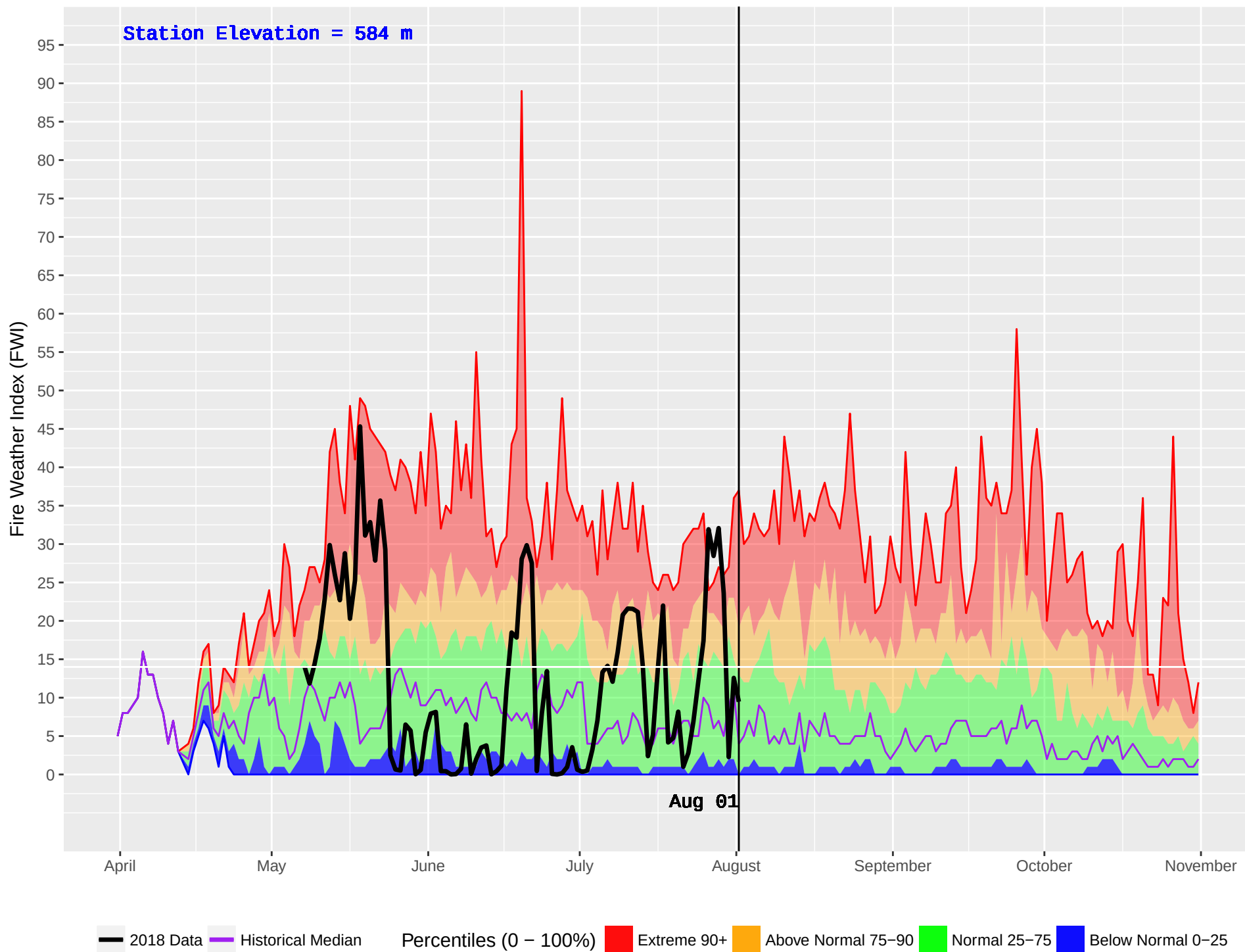
SIERRA (117) : Historical (1981–2016) and Current (2018) Daily Fire Weather Index (FWI)
