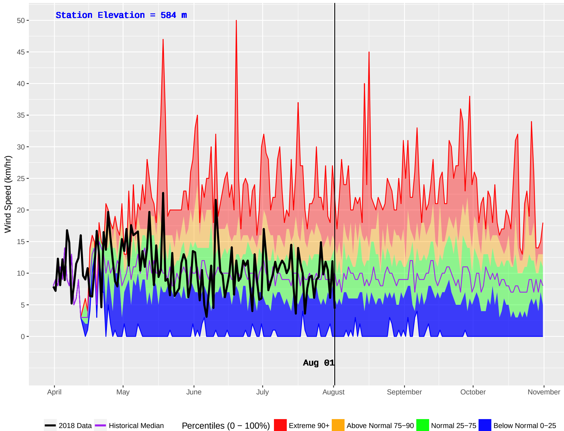
SIERRA (117) : Historical (1981–2016) and Current (2018) Daily Wind Speed
