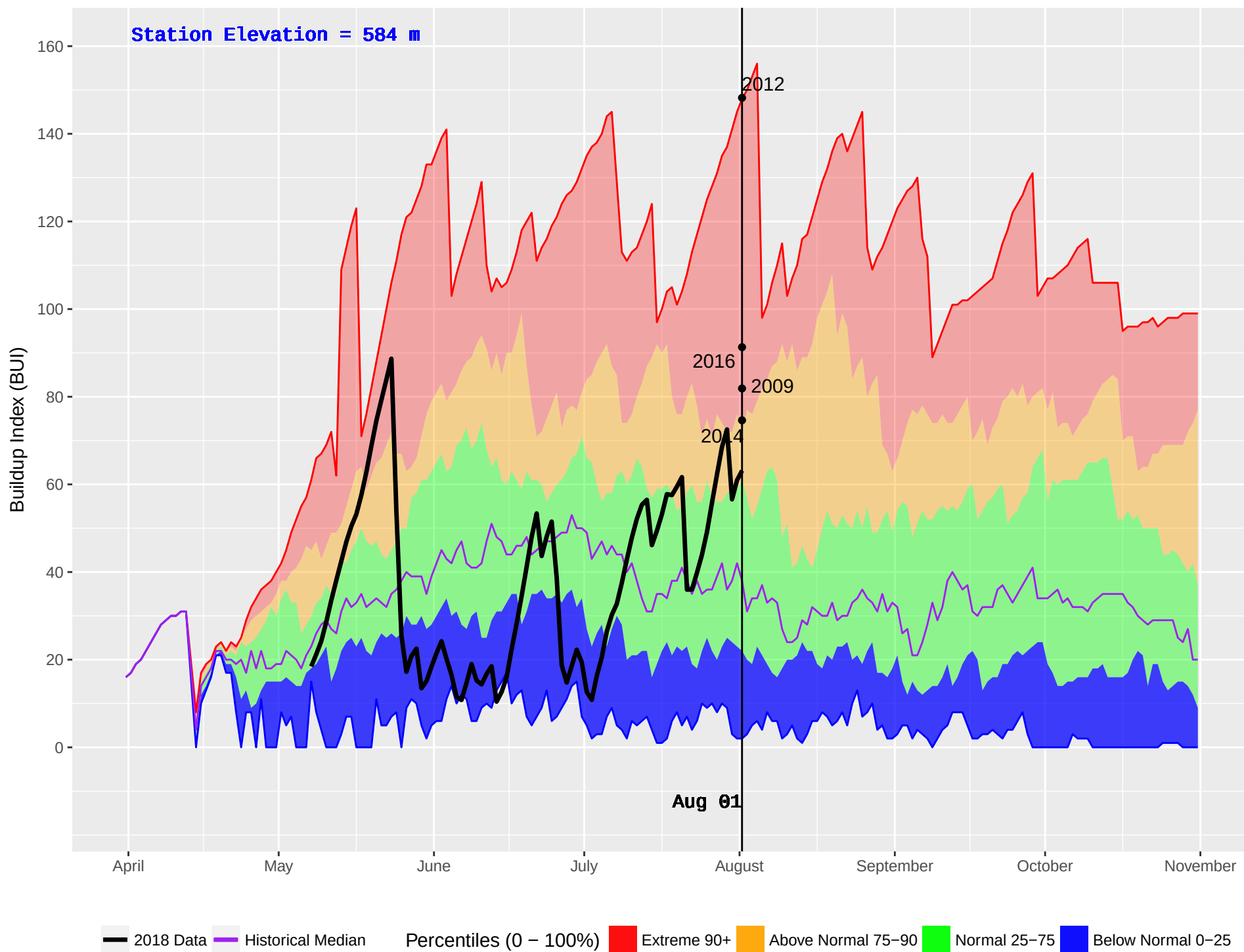
SIERRA (117) : Historical (1981–2016) and Current (2018) Daily Buildup Index (BUI)
