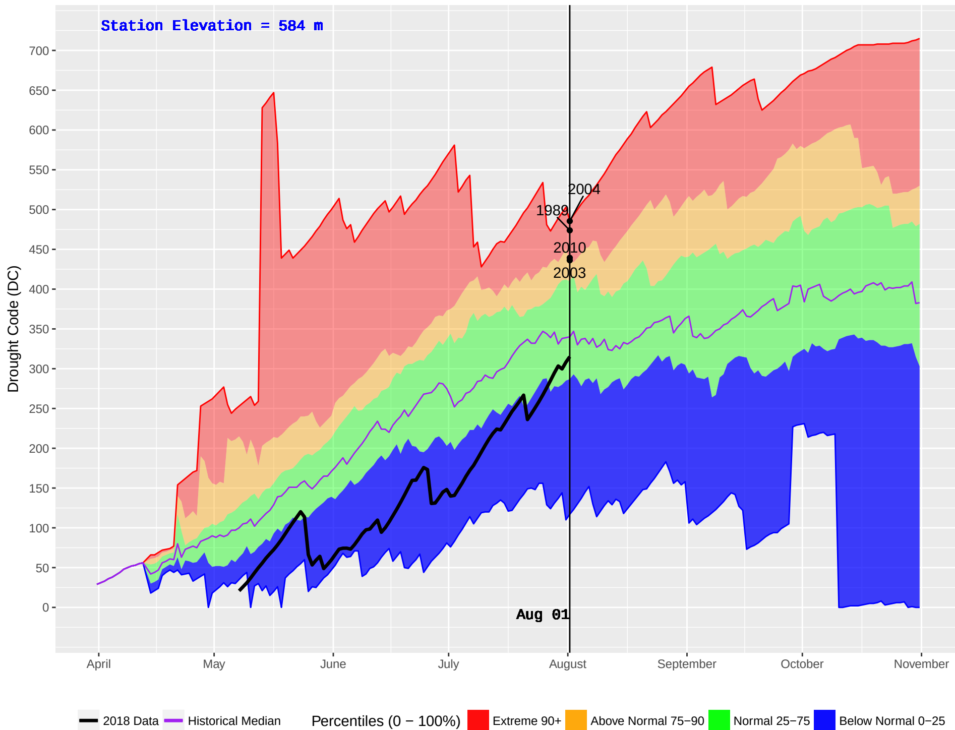
SIERRA (117) : Historical (1981–2016) and Current (2018) Daily Drought Code (DC)
